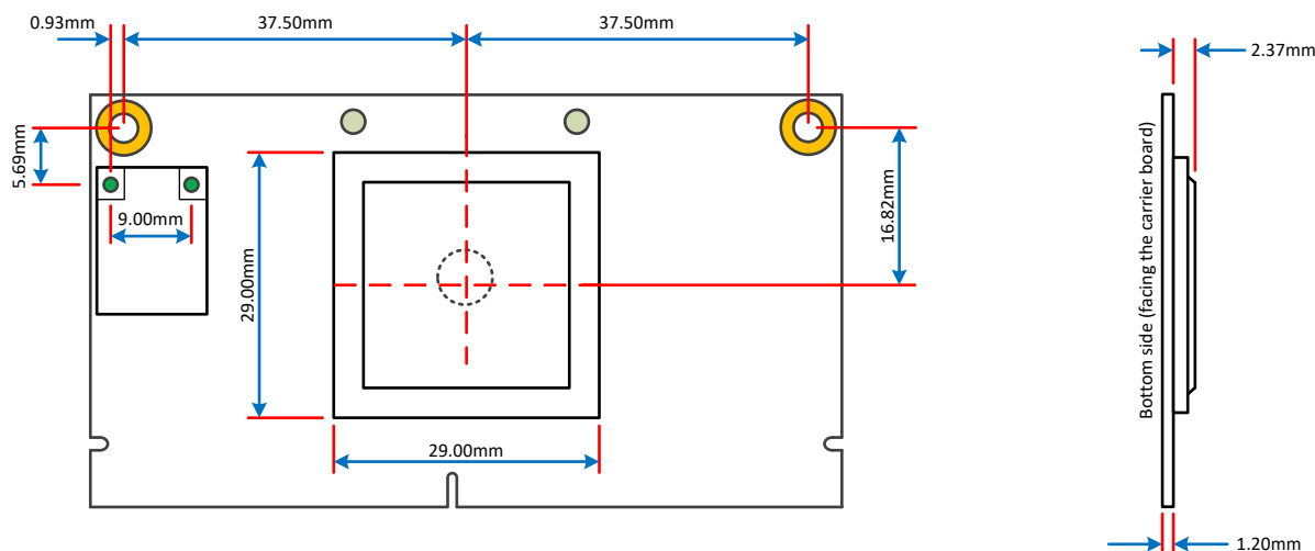
Figure 21 Mechanical position of i.MX 8 SoC (top view) Tolerance for all measures: +/- 0.1mm
